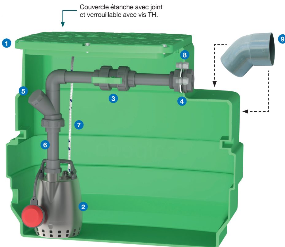
CAL230 GXRM 10-9
