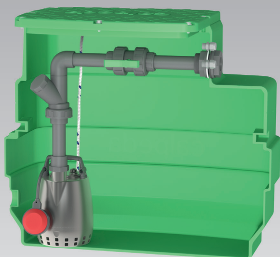
CAL230 GXRM 10-9
